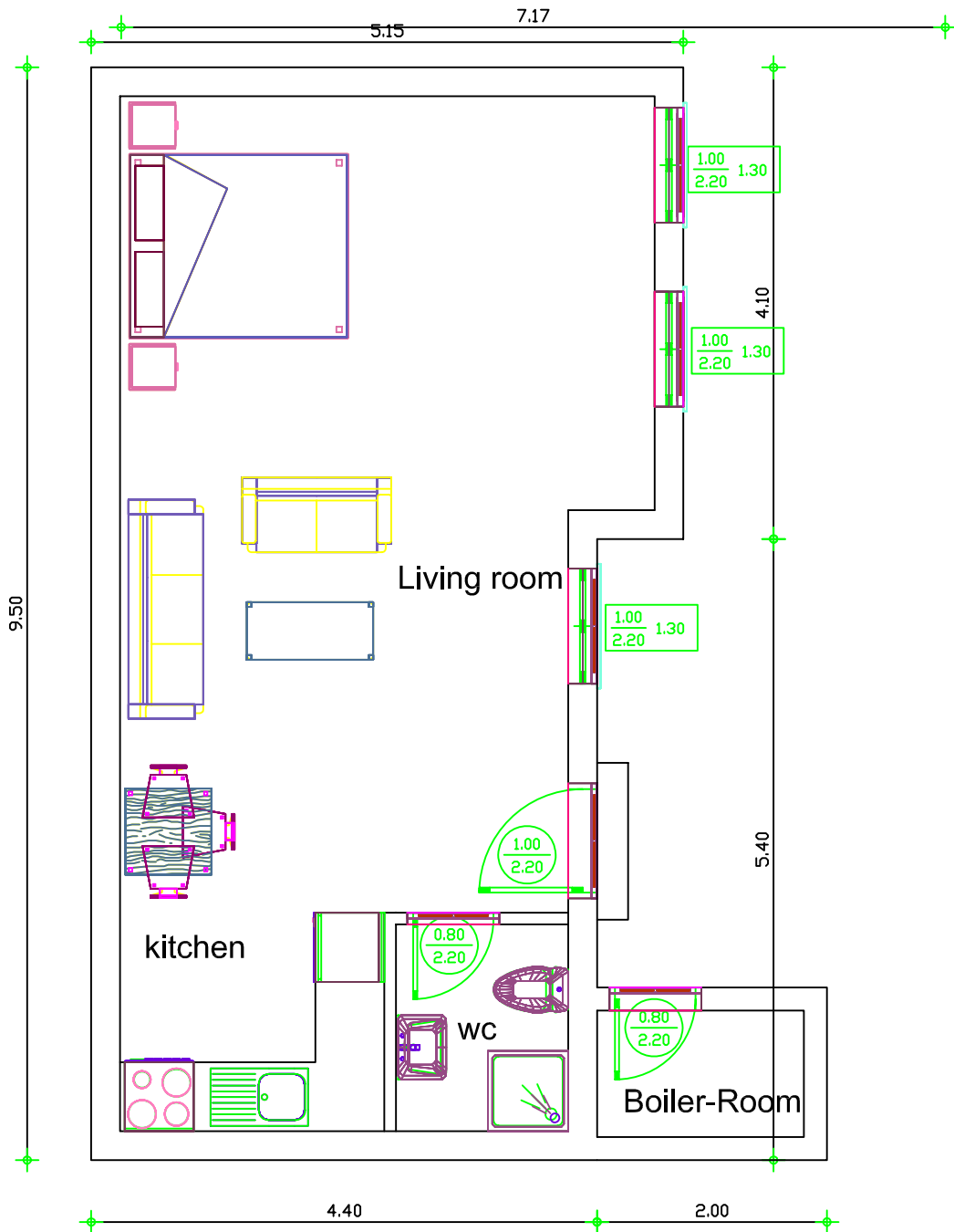
2 - First Floor Floor area =45.00 m2
